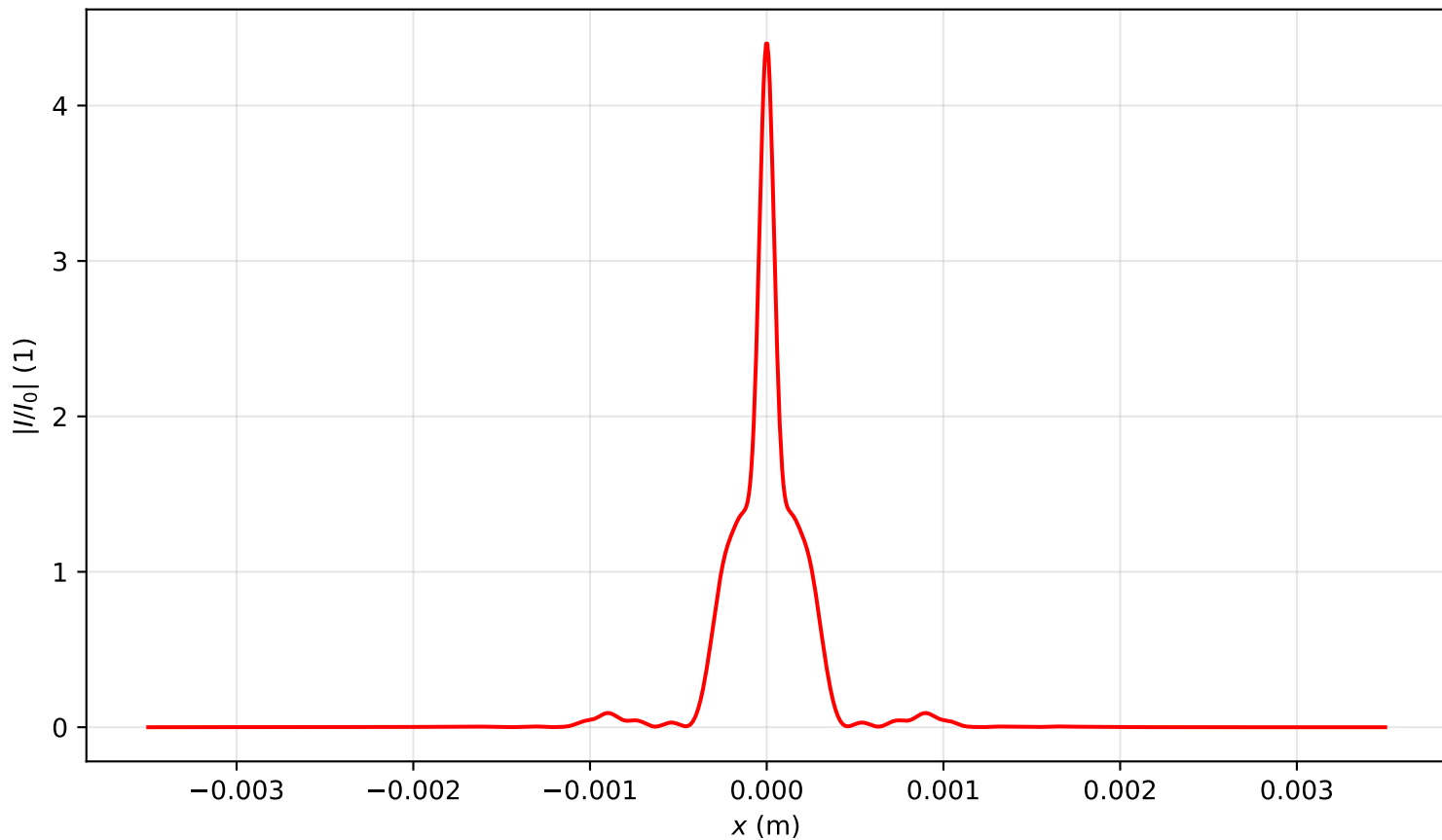
Intensity profile I(x, y = 0, z = 1.194)/I_0 , P_{in}=5.0P_{cr} , artificial time
